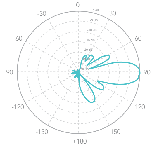
Horizontal Elevation
